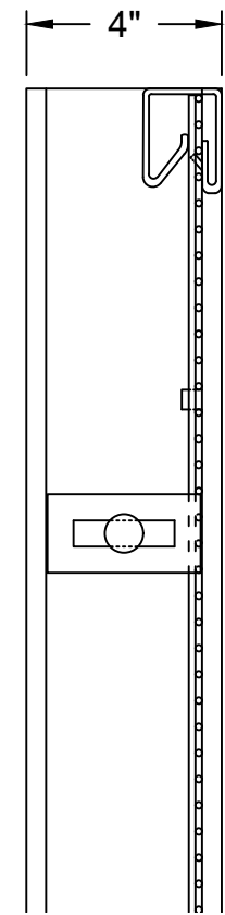
SECTION A
